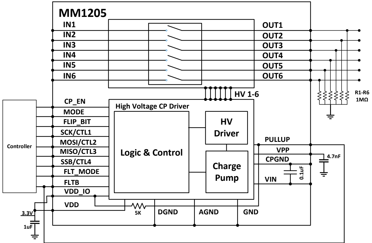
Figure 23. MM1205 Application Diagram
