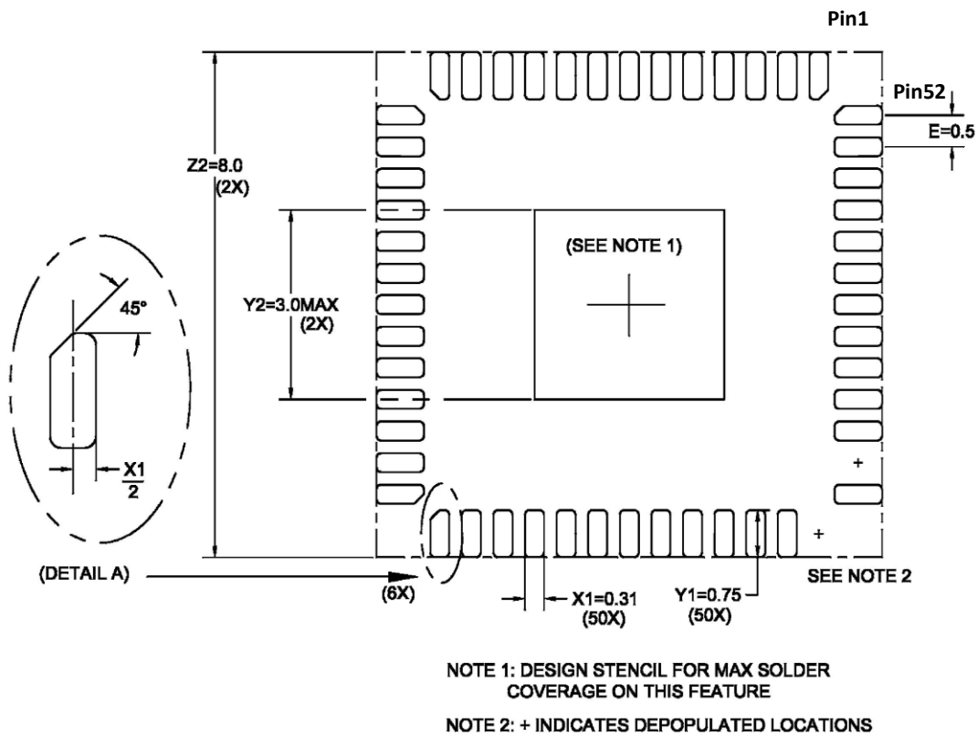
Figure 25. Recommended PCB Pad Pattern Top View
