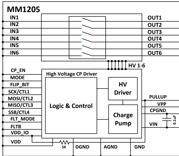
Figure 4. Functional Block Diagram (IN x = Contact, OUT x = Beam)
