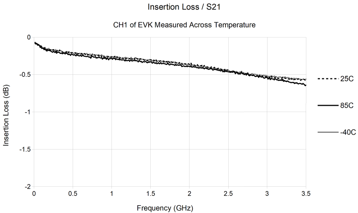
Figure 10. Typical Channel Insertion Loss vs Frequency ( S_{21} )
