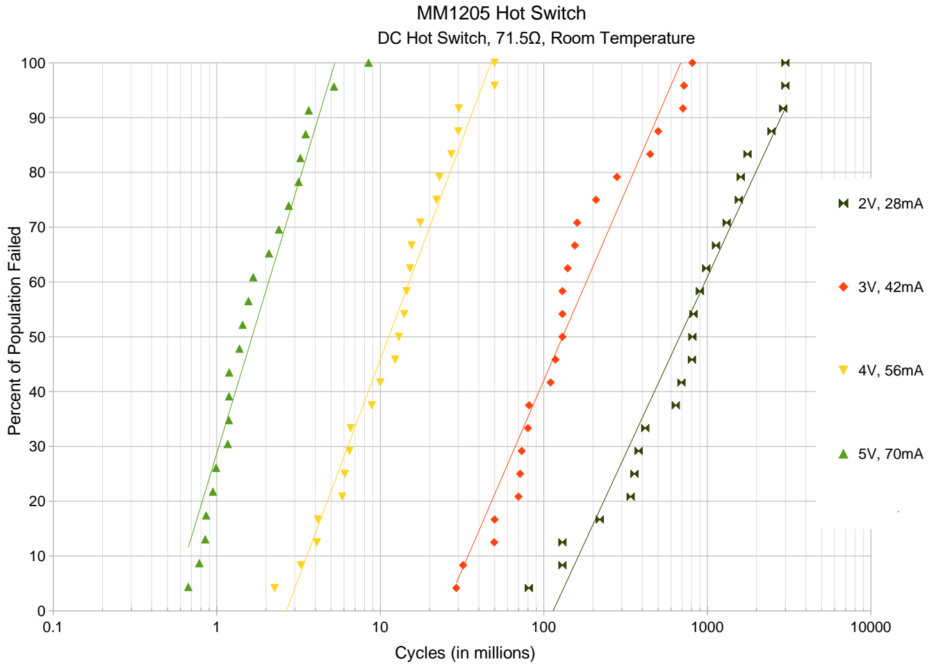
Figure 15. Hot Switch Endurance Test Results
