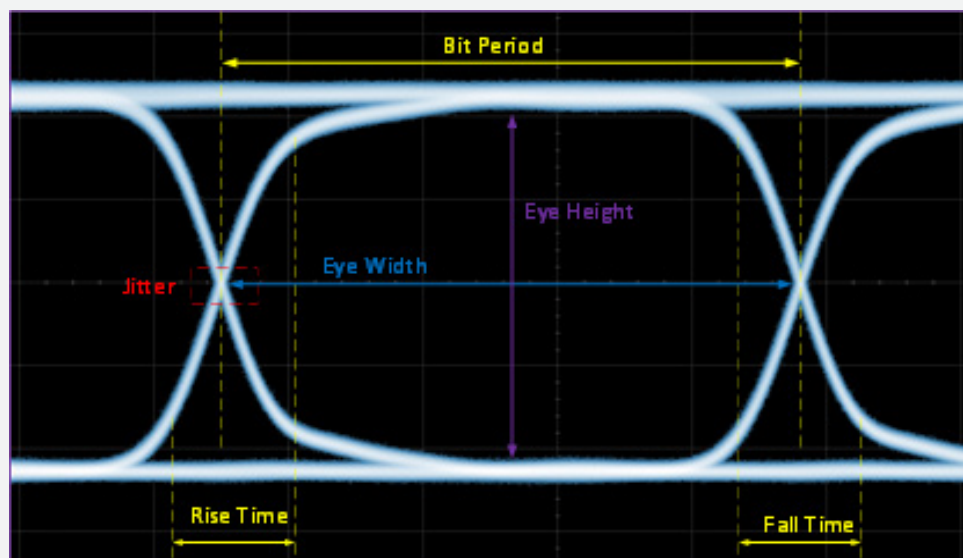
FIG. 2 Eye Diagram Measurement
