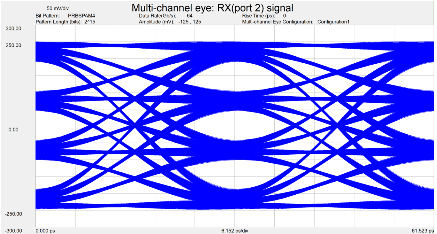
Figure 1. HS1-HS2 Differential PAM4 Eye Diagram
