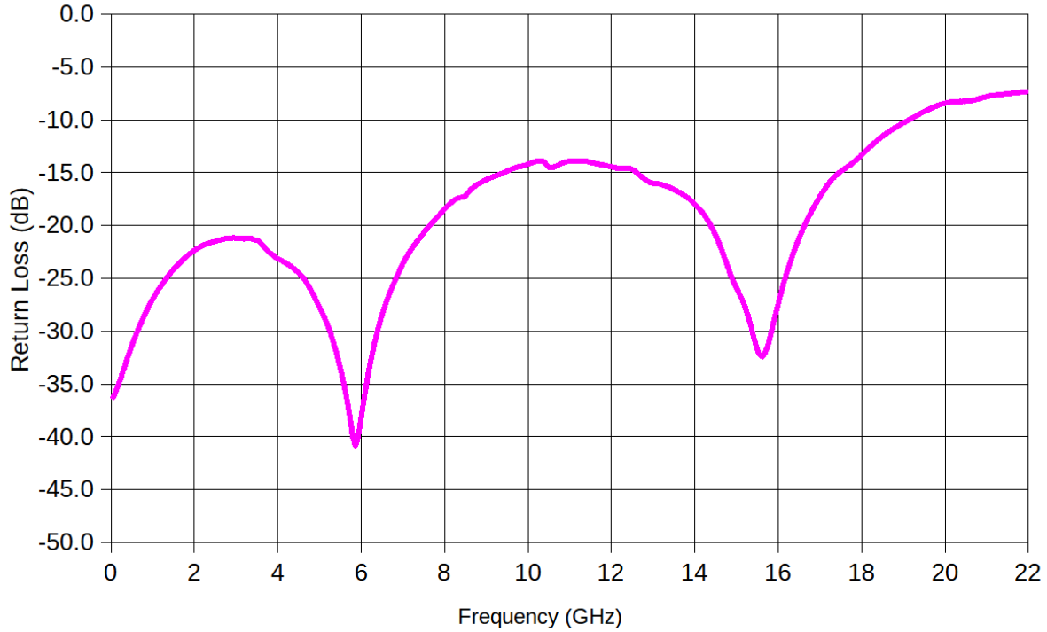
Figure 6. Return Loss/SDD11
