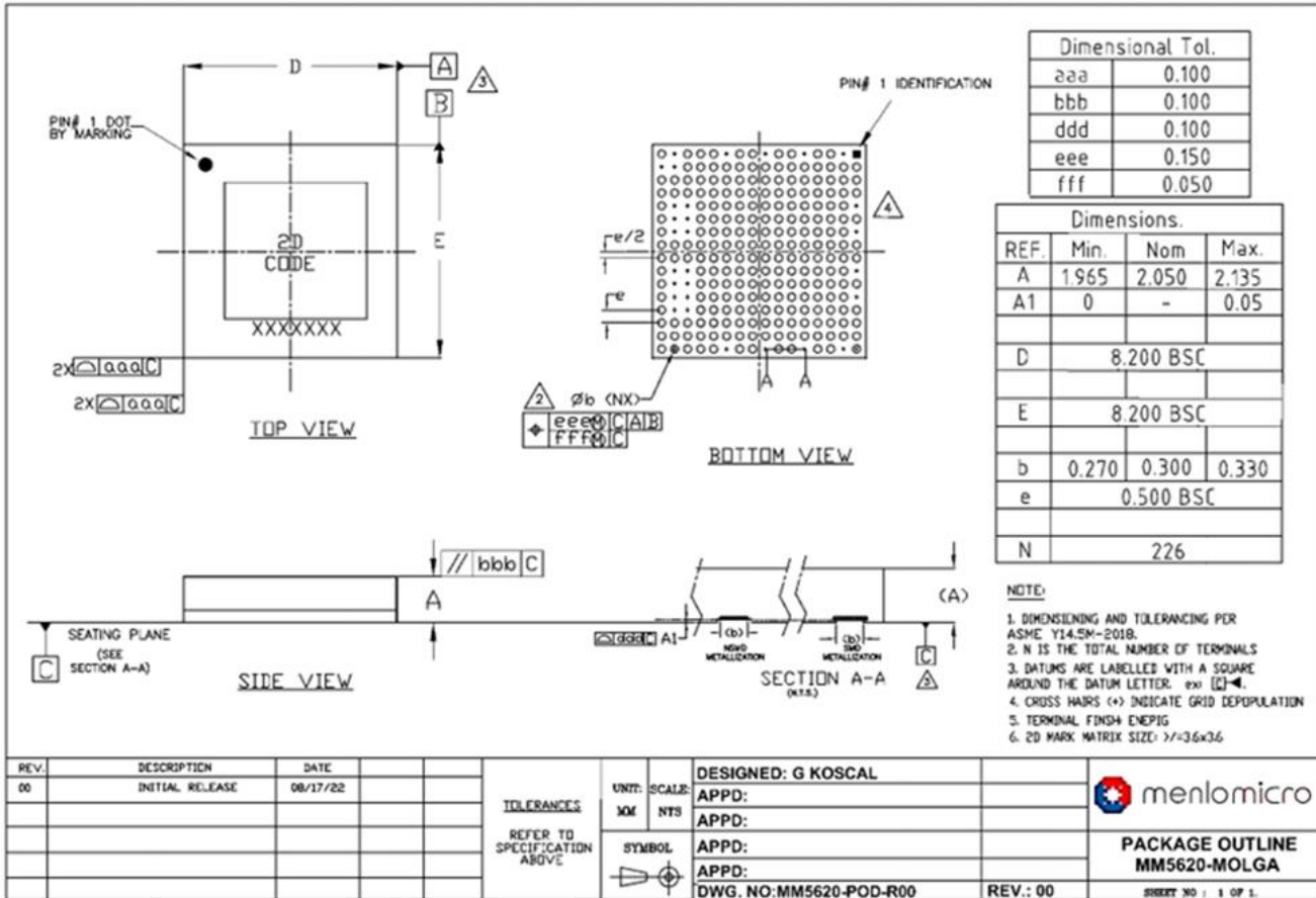
Figure 18. Package Drawing
