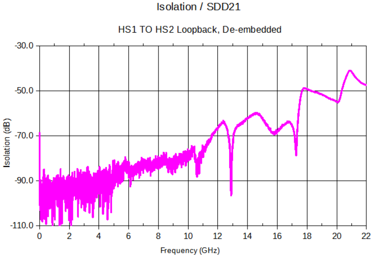
Figure 7. Isolation/SDD21
