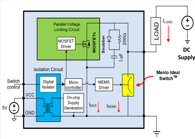
FIG. 1 MM9105-DC Relay
