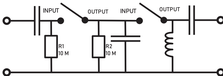
Figure 2: L-C Network from Figure 1 with Added Resistors Eliminates the Isolated Nodes
